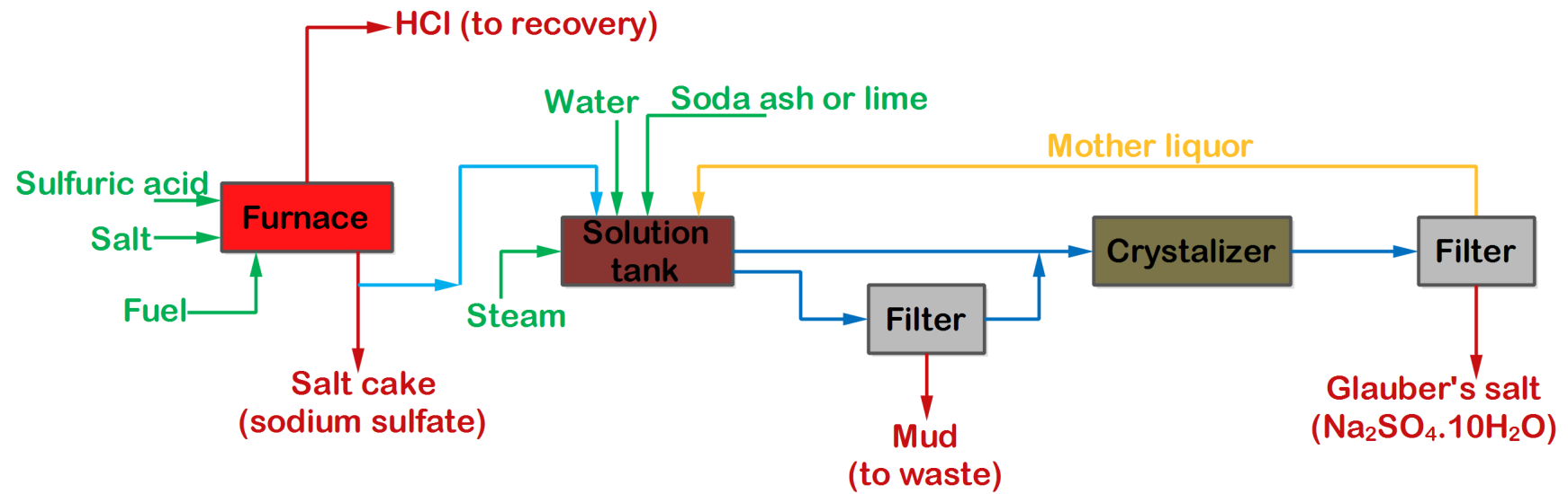
Figure: Manufacture of Sodium sulfate from salt and sulfuric acid
